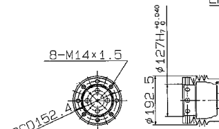
CRANK PULLEY DETAIL
